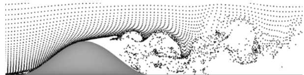
(b) Numerical simulation (RIAM-COMPACT®), passive particle tracking method
