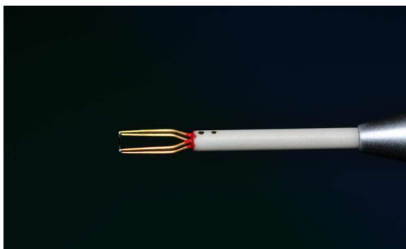
Fig. 6 Split-fiber probe, capable of detecting reversed flow
